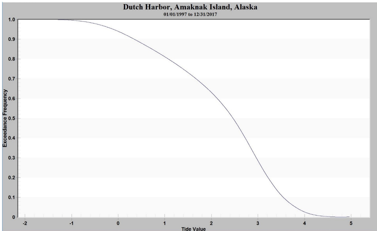
Figure 11. Tidal Exceedance Function for Dutch Harbor 1997-2017
