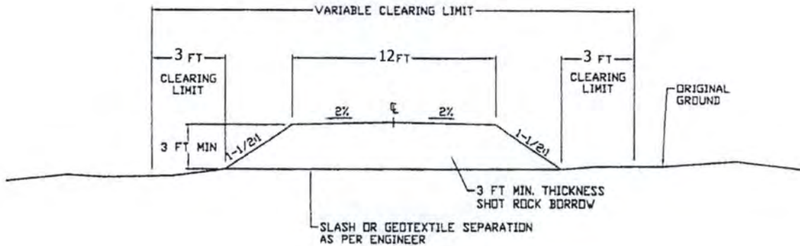
TYPICAL OVERLAY SECTION (NTS)
