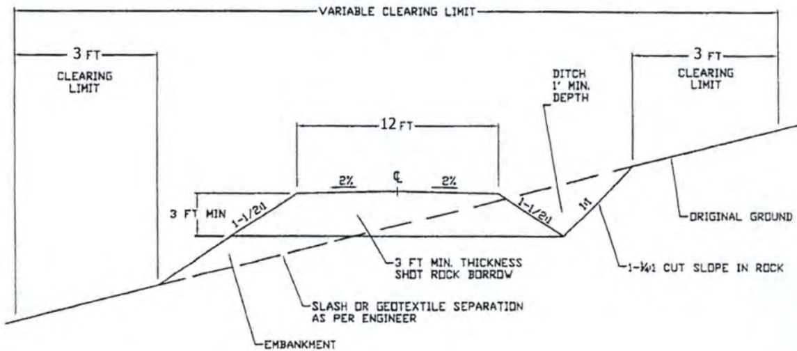
TYPICAL BALANCED CUT/FILL SECTION (NTS)
