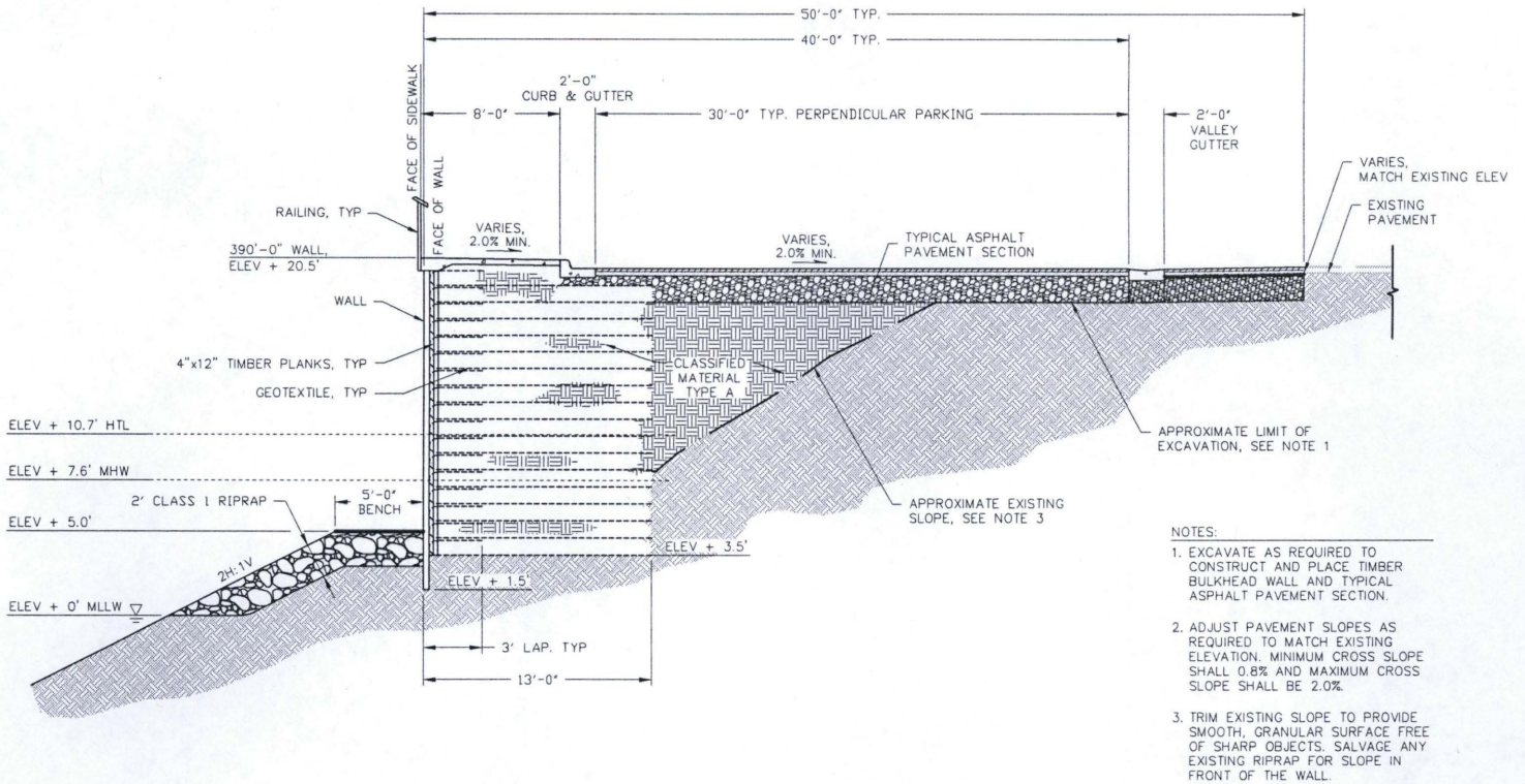
1 TYPICAL BULKHEAD PARKING AREA SECTION 4 NTS STATION 10+15.00 TO STATION 13+80.58
