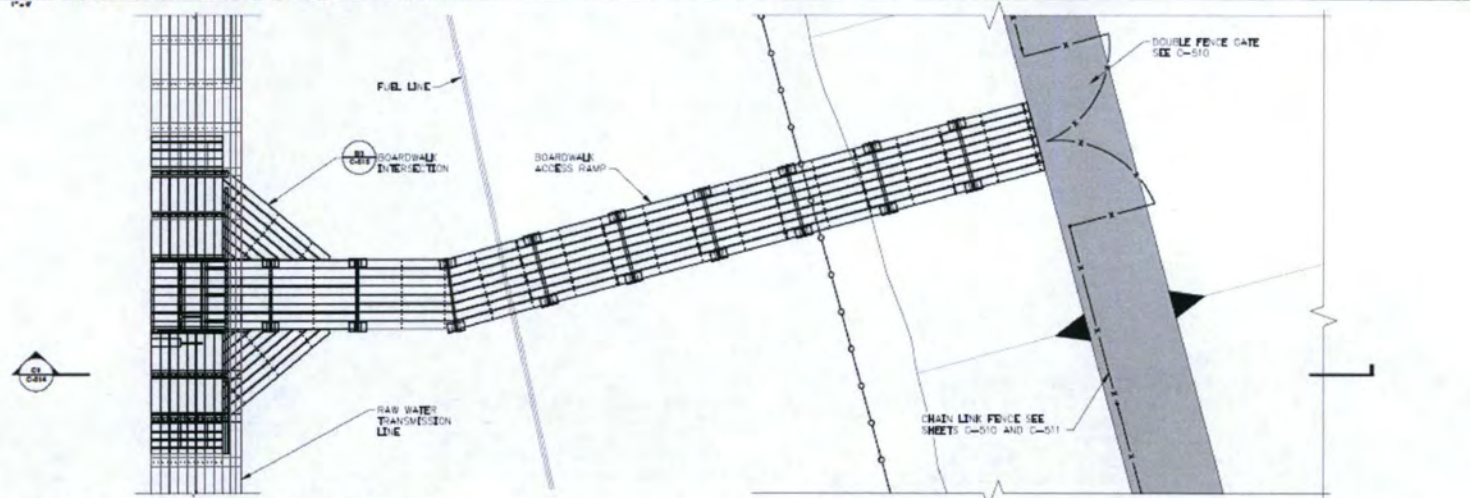
A1 LAGOON ACCESS BOARDWALK RAMP - PLAN 1"=8'
