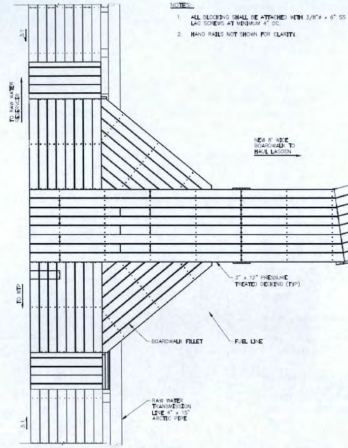
B3 PLAN VIEW - BOARDWALK 1"=1'
