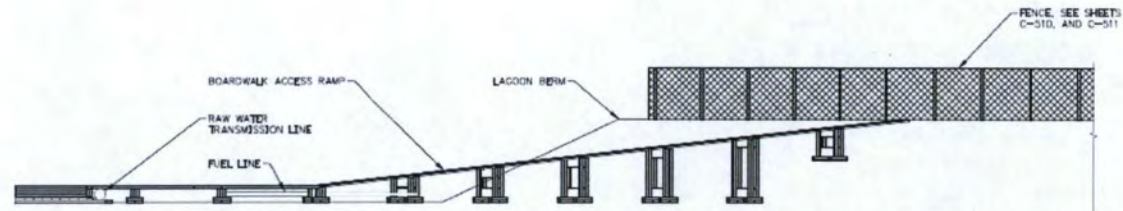
C1 LAGOON ACCESS BOARDWALK RAMP - SECTION 1"=8'
