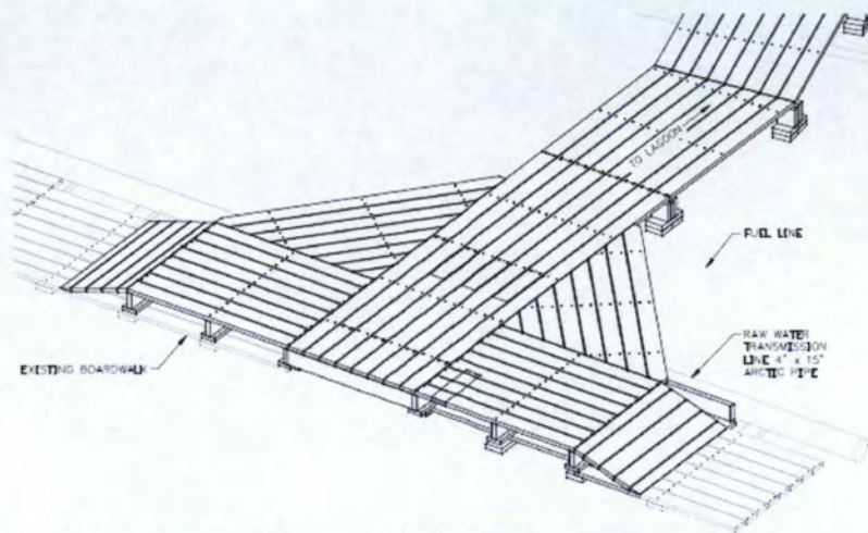
C1 BOARDWALK INTERSECTION SW ISOMETRIC VIEW 1"=1'
