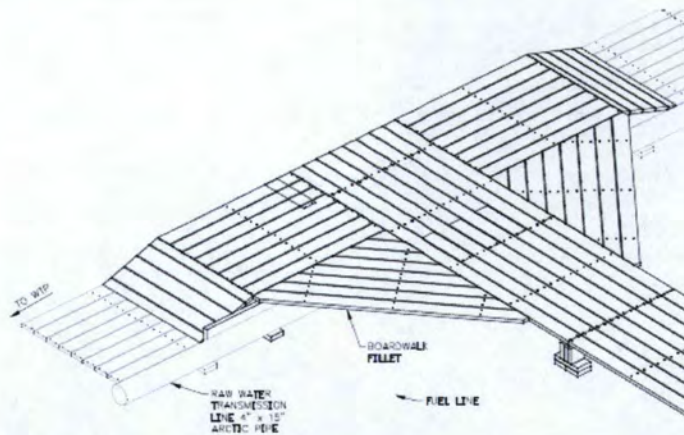
A1 BOARDWALK INTERSECTION SE ISOMETRIC 1"=1'
