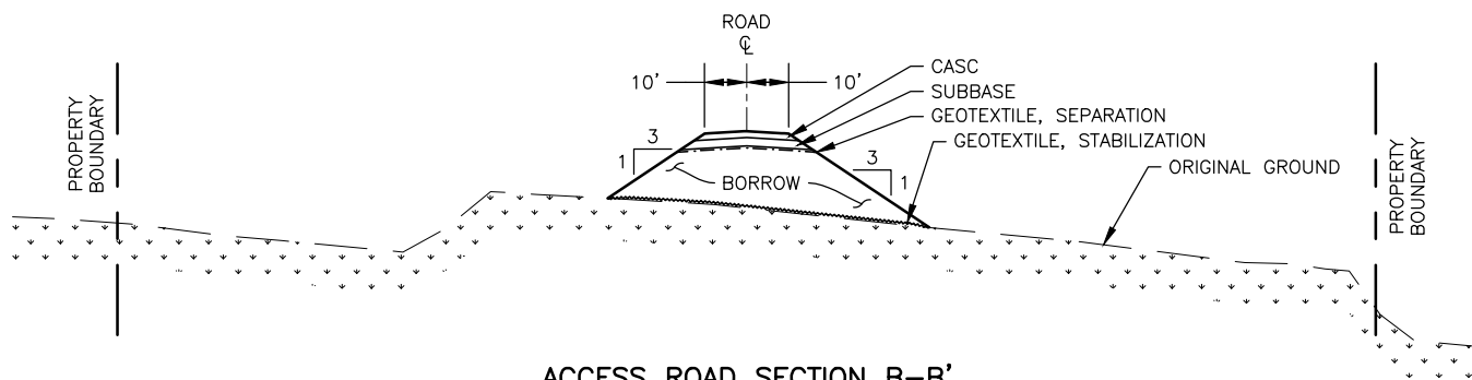
ACCESS ROAD SECTION B-B' NTS
