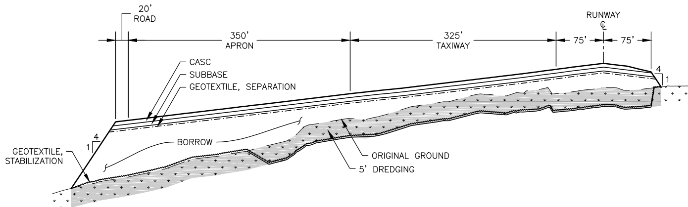
AIRPORT SECTION A-A' NTS
