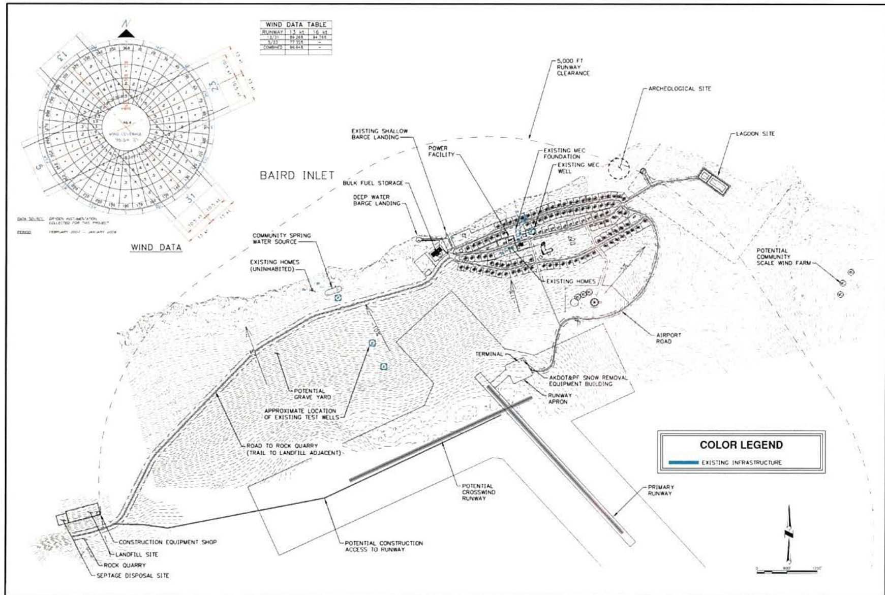
Figure 3. FEIS Mertarvik Preferred Alternative Airport Configuration
