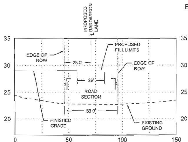
ROAD SECTION B-B'
