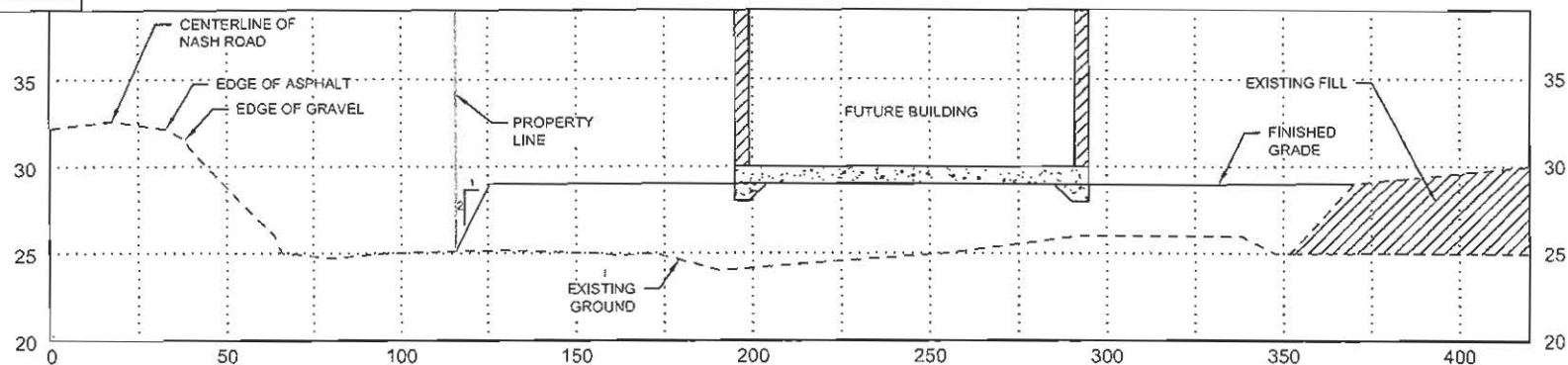
BUILDING PAD SECTION A-A'
