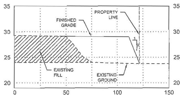
STORAGE PAD SECTION C-C'
