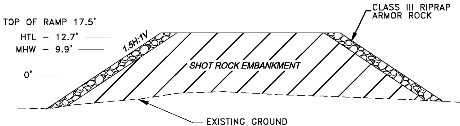
TYPICAL RAMP SECTION 1"=20'
